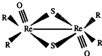
\text{R} = \text{CH}_2\text{CMe}_3 (5)
